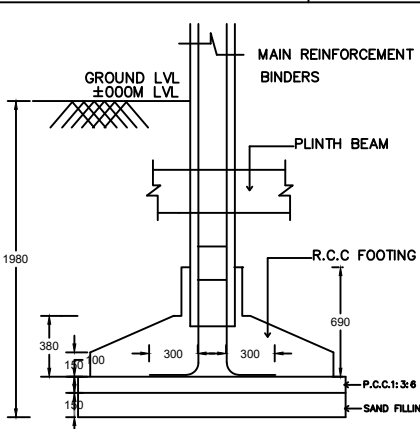
TYPICAL SECTION OF R.C.C COLUMN FOUNDATION SCALE : 1" = 2'-0"
