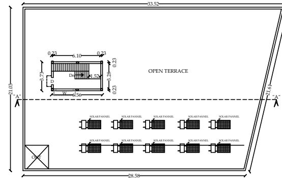
TERRACE FLOOR
