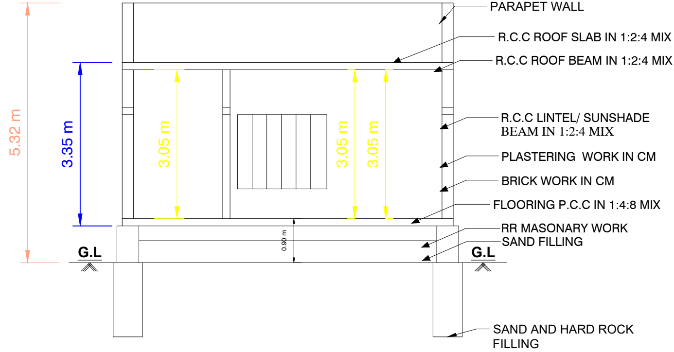
SECTION"AB"
