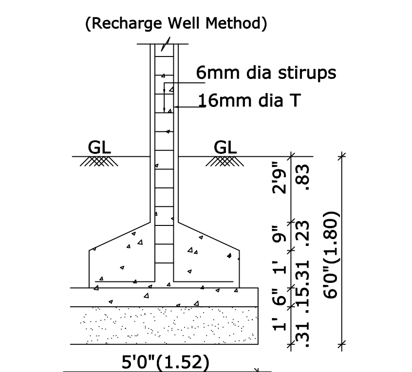
COLUMN FOUNDATION DETAIL
