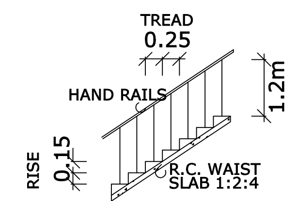
STAIRCASE DETAILS
