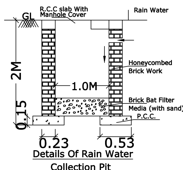
Details Of Rain Water Collection Pit
