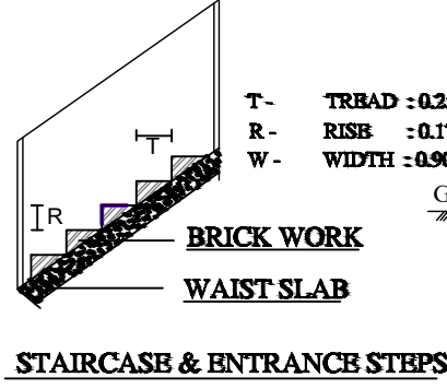
STAIRCASE & ENTRANCE STEPS
