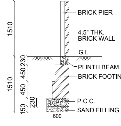
DETAILS OF COMPOUND WALL
