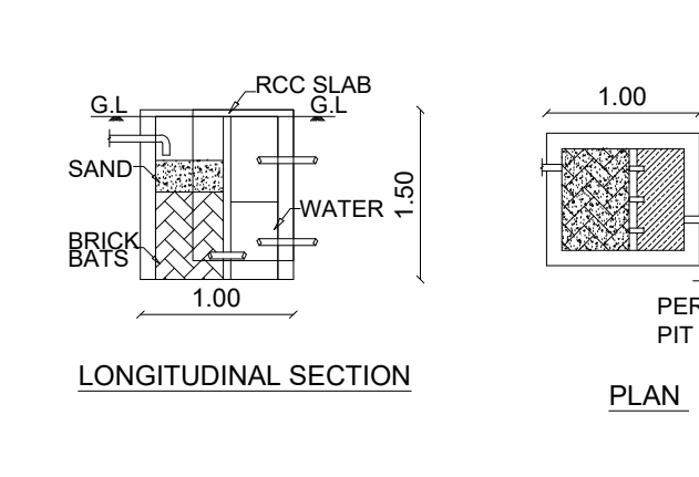
RAIN WATER HARVESTING FILTER BED
