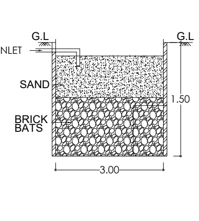
RAIN WATER HARVESTING NOT TO SCALE
