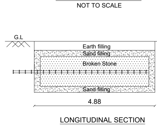
DISPERSION TRUNCH NOT TO SCALE
