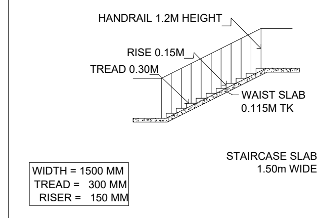
DETAILS OF STAIRCASE SCALE 1:50
