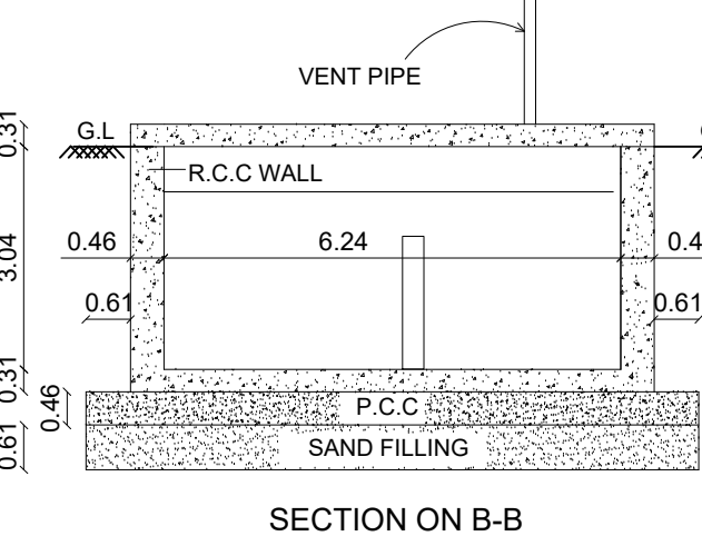
DETAILS OF SEPTIC TANK SCALE - 1:30
