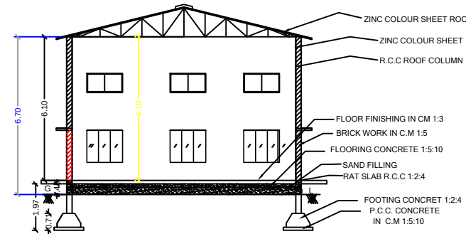
SECTION - XX
