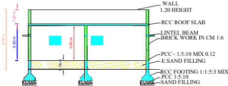
SECTION ON "AB"
