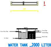
WATER TANK _2000 LITER
