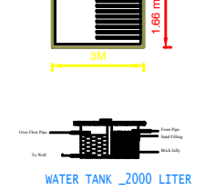
WATER TANK 2000 LITER
