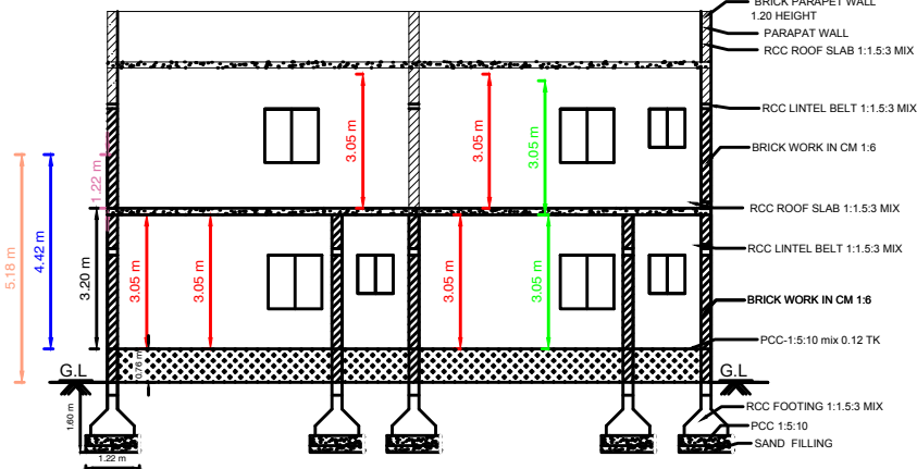
SECTION " AB "
