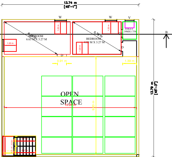
RESIDENTIAL PLAN FIRST FLOOR
