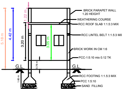
SECTION " AB "
