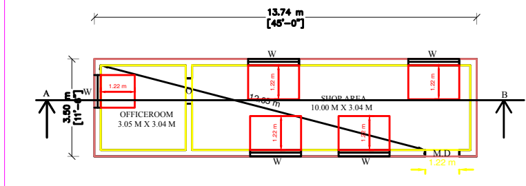
COMMERCIAL PLAN
