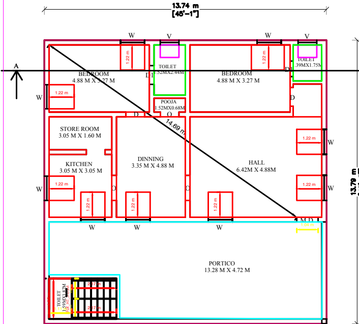
RESIDENTIAL PLAN GROUND FLOOR
