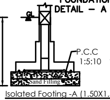
FOUNDATION DETAIL - A (Not To Scale)
