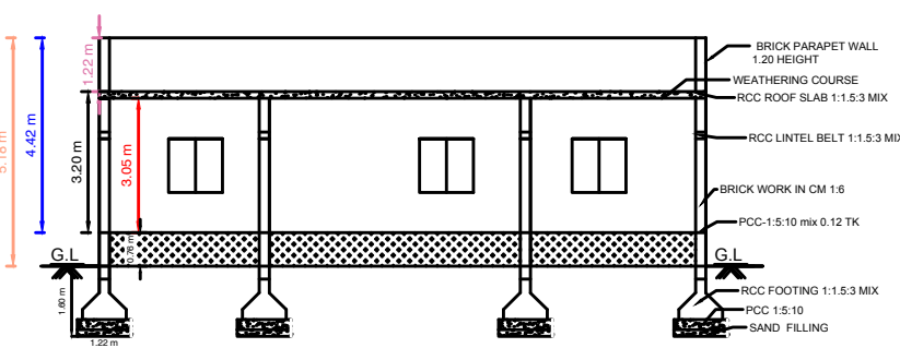
SECTION " AB "
