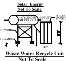
Waste Water Recycle Unit Not To Scale
