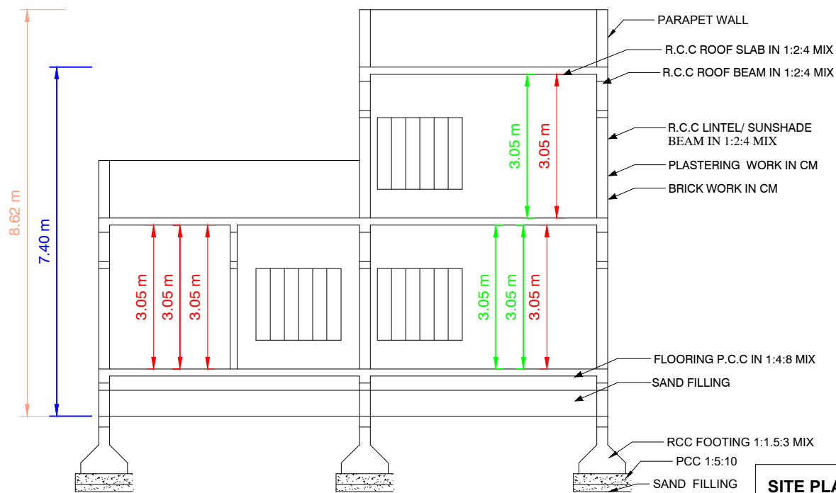
SECTION"AB"
