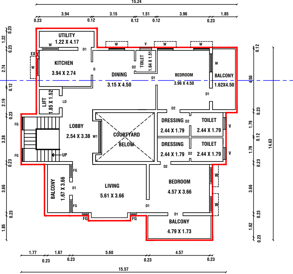
FLOOR - FIRST
