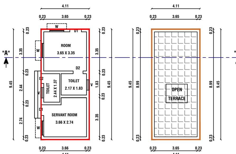
BLOCK-2 PRO. GROUND FLOOR PLAN
