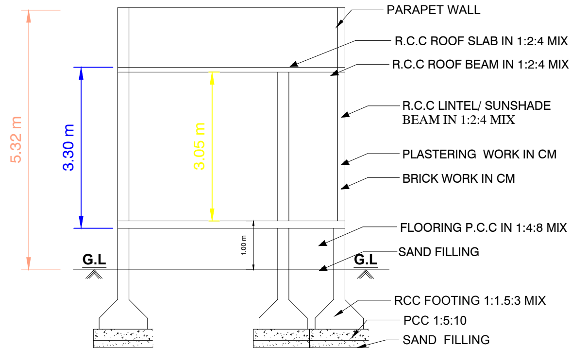
SECTION"AB"
