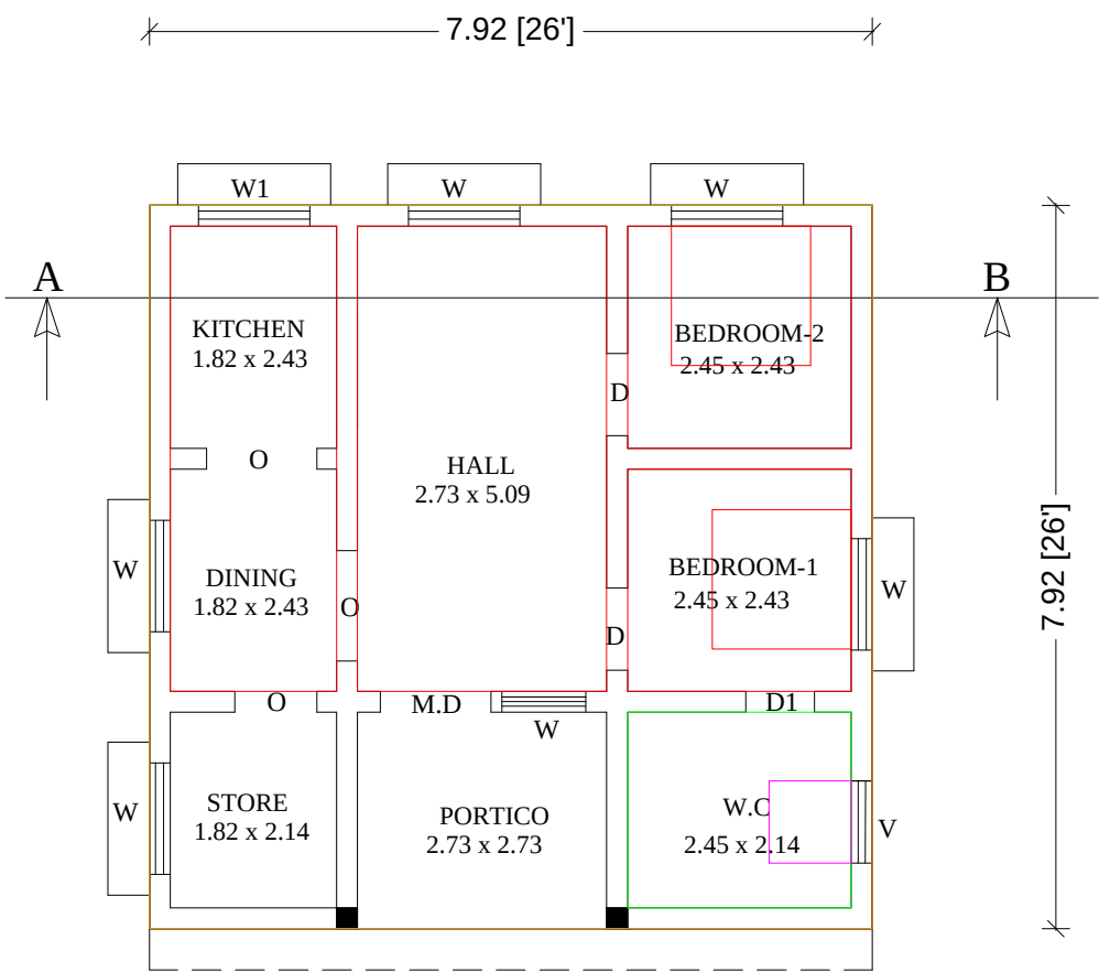
GROUND FLOOR
