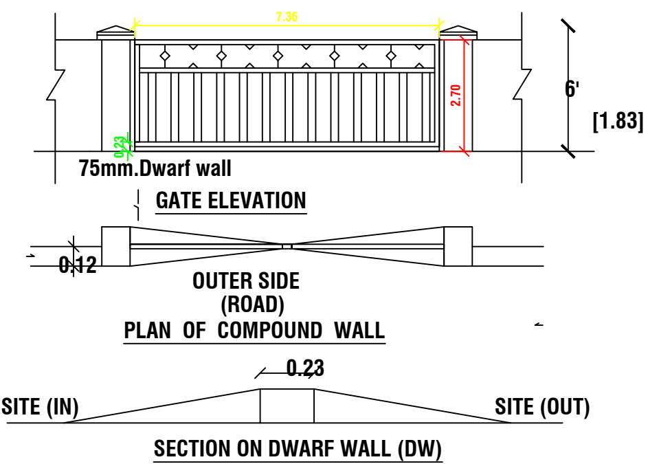
PLAN OF COMPOUND WALL SECTION ON DWARF WALL (DW)
