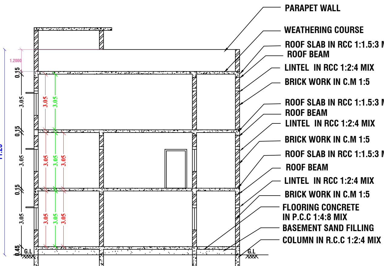
SECTION "A-A"
