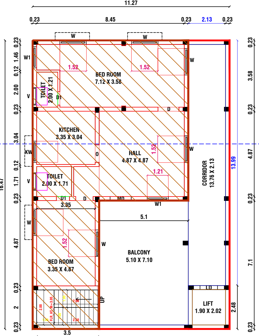
FLOOR - FIRST PRO. FIRST FLOOR PLAN
