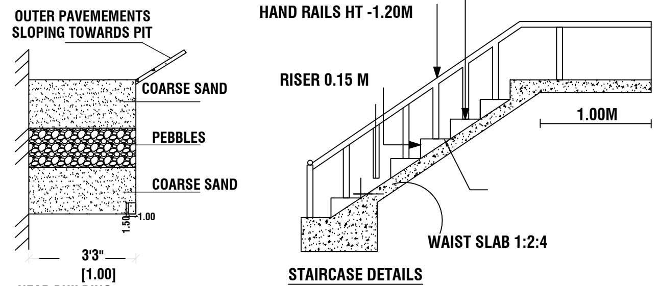
STAIRCASE DETAILS
