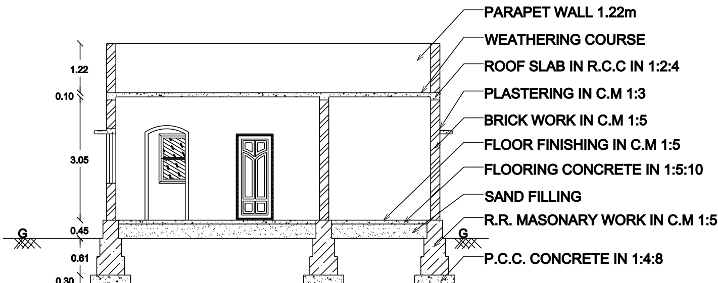
SECTION "XY"
