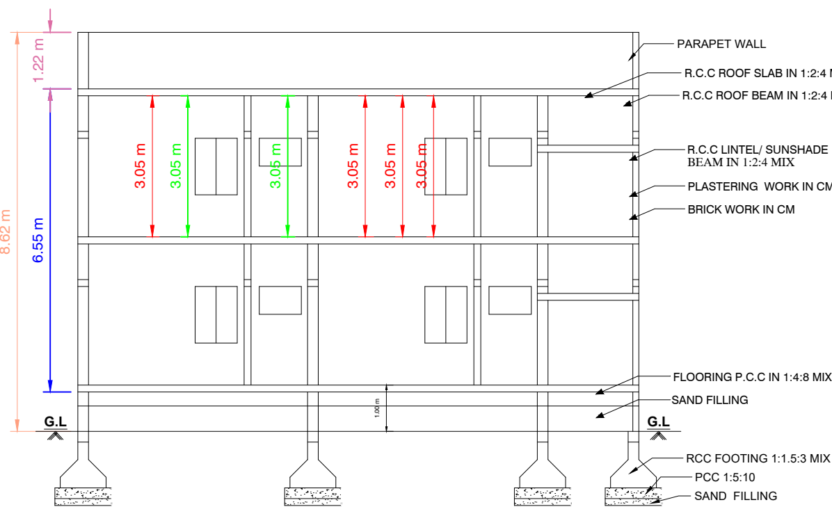
SECTION"AB"
