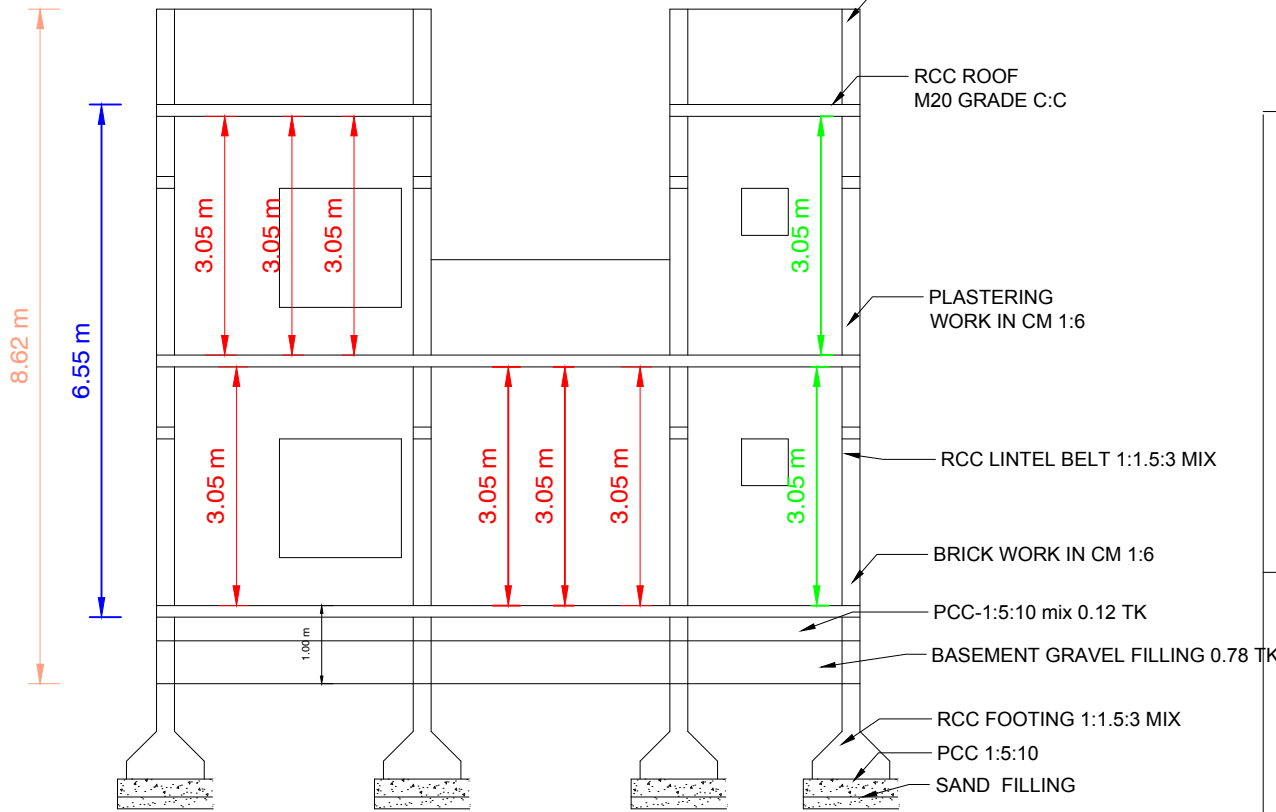
SECTION"AB"
