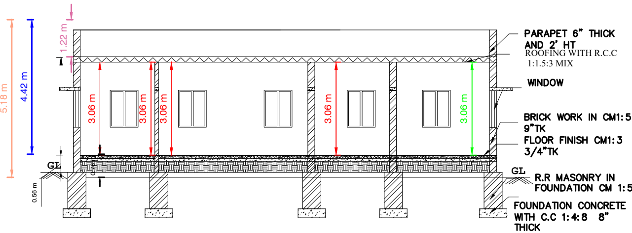
SECTION " AB "
