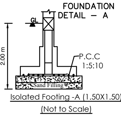
FOUNDATION DETAIL - A (Not to Scale)
