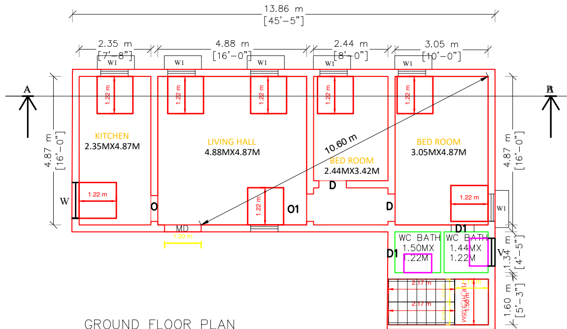
GROUND FLOOR PLAN ENTRANCE FACING TO NORTH
