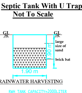
RAINWATER HARVESTING RWH TANK CAPACITY=2000LITER
