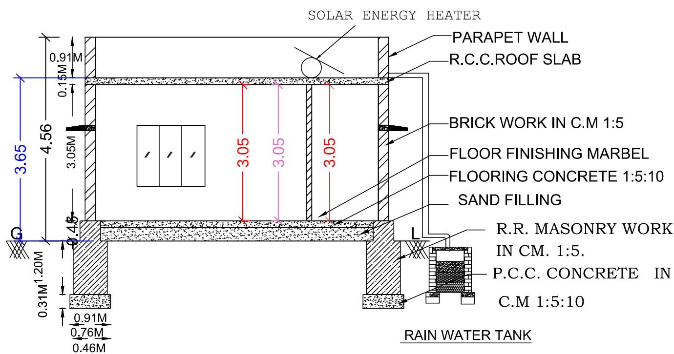
SECTION - XX
