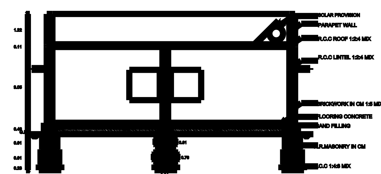
SECTION ON 'ABC'
