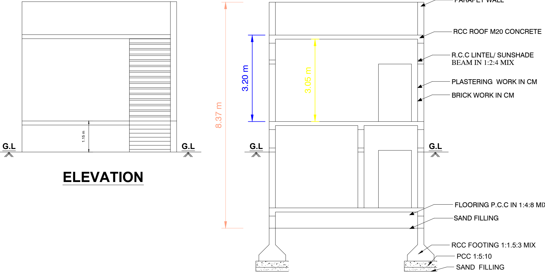
SECTION"AB"
