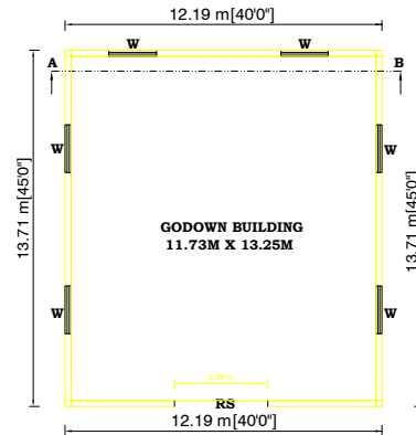
GODOWN BUILDING - PLAN
