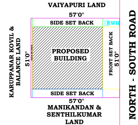
RAINWATER HARVESTING RWH TANK CAPACITY=2000LITER
