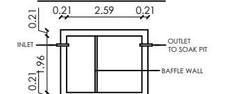
PLAN SEPTIC. TANK
