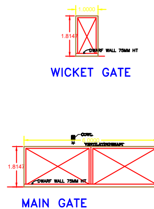
MAIN GATE
