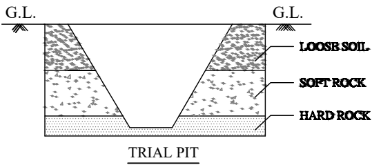
TRIAL PIT
