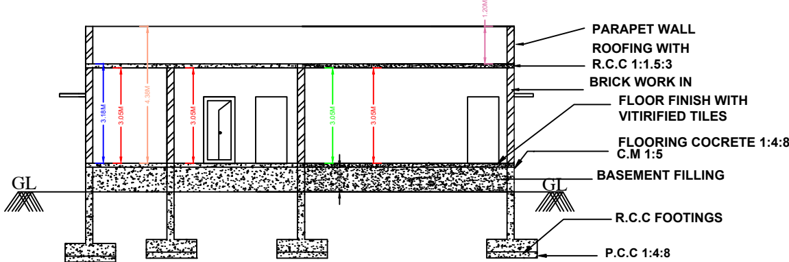
SECTION ON "BB1"
