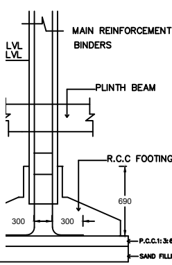
TYPICAL SECTION OF R.C.C. COLUMN FOUNDATION SCALE : 1" = 2'-0"
