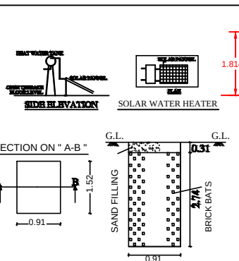
DETAILED PLAN OF RAINWATER COLLECTION AND CIRCULATION PIT
