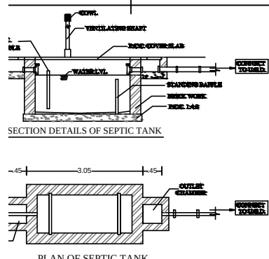
SECTION DETAILS OF SEPTIC TANK
