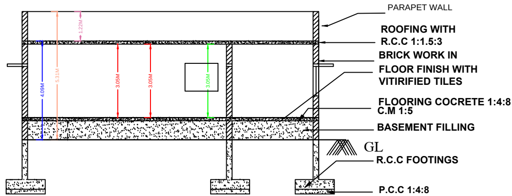
SECTION ON "BB1"
