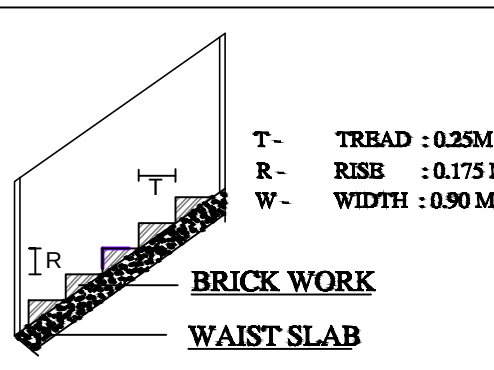
STAIRCASE & ENTRANCE STEPS
