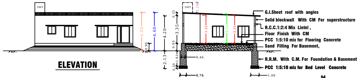
SECTION ON "XY"
