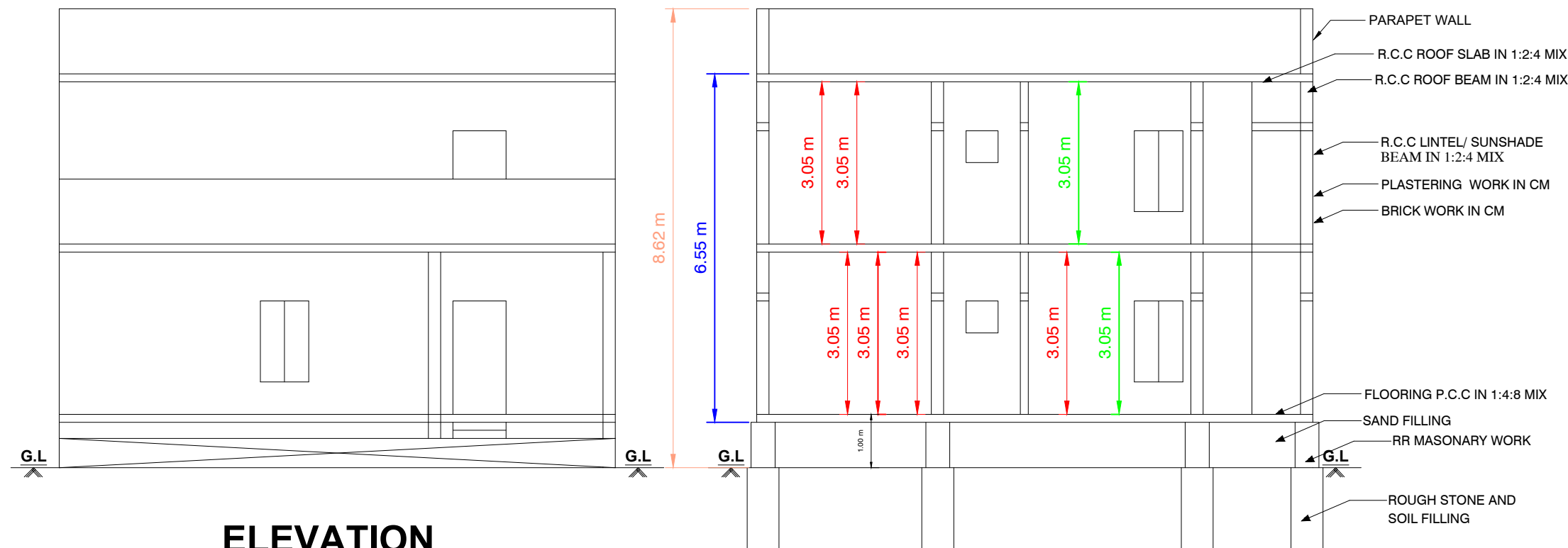
SECTION"AB"
