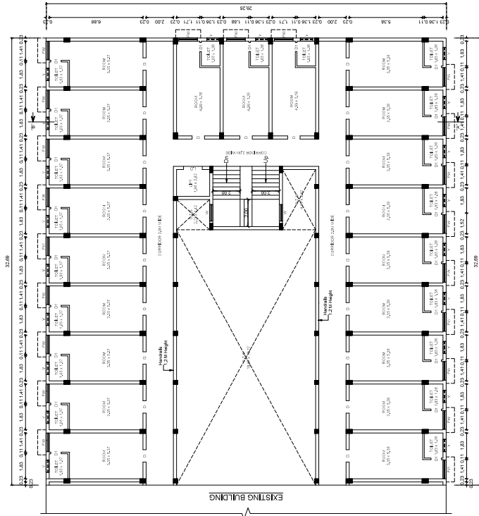
TYPICAL FLOOR PLAN - FIRST, SECOND, THIRD AND FOURTH FLOOR
