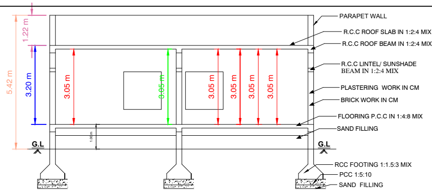
SECTION"AB"
