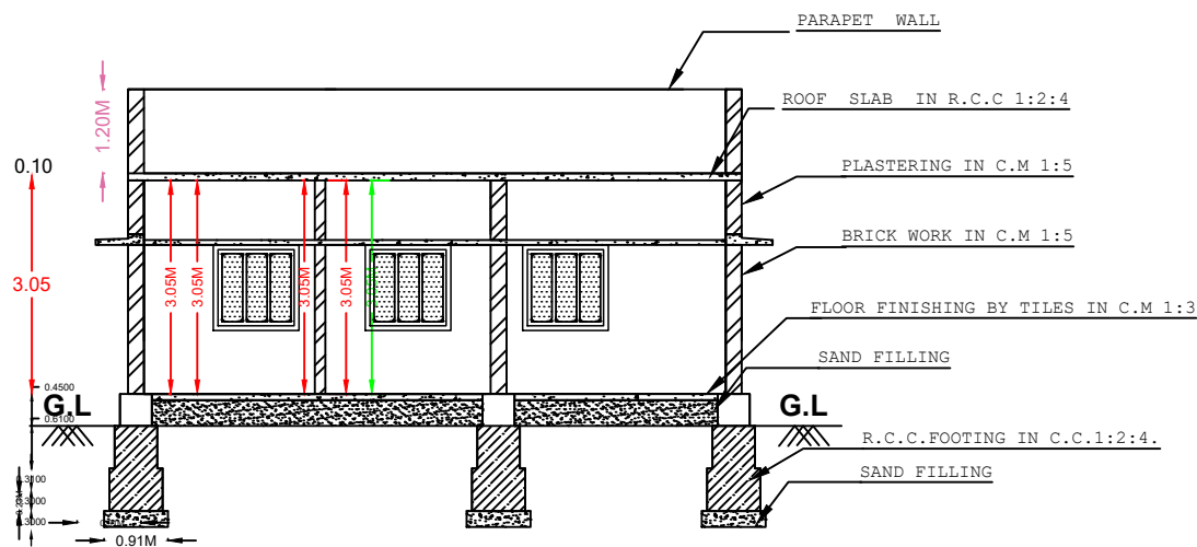
SECTION ON - XY.
