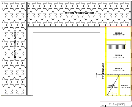
PROPOSED FIRST FLOOR [WEST PART] -COMMERCIAL - PLAN
