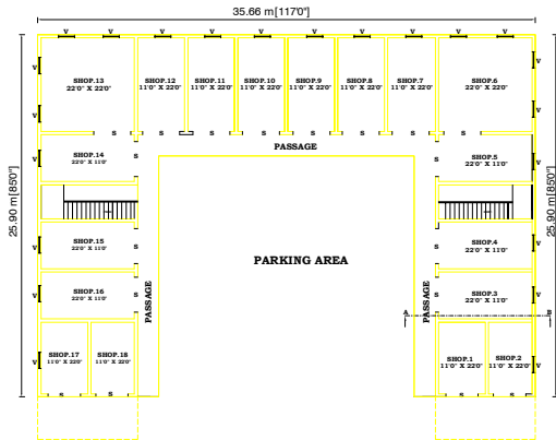
EXISTING GROUND FLOOR -COMMERCIAL - PLAN
