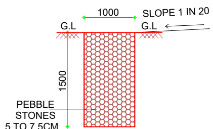
RAIN WATER COLLECTION PIT
