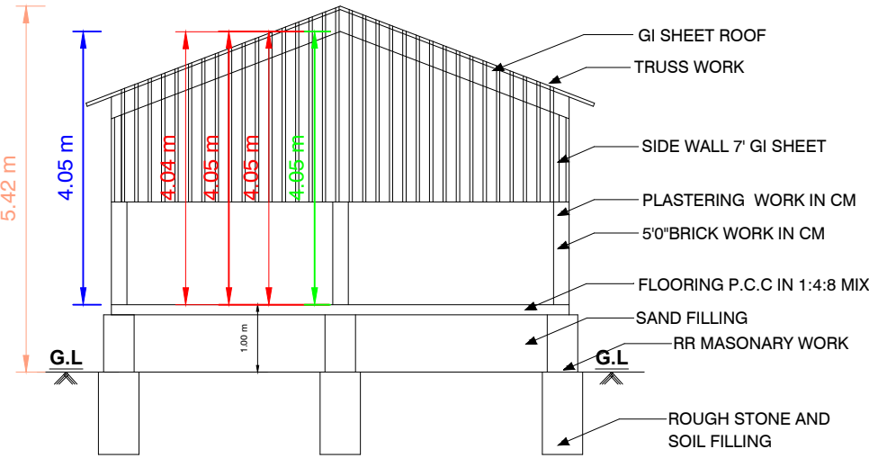
SECTION"AB"
