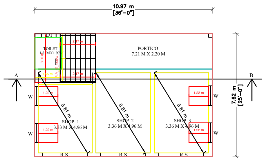
COMMERCIAL PLAN GROUND FLOOR
