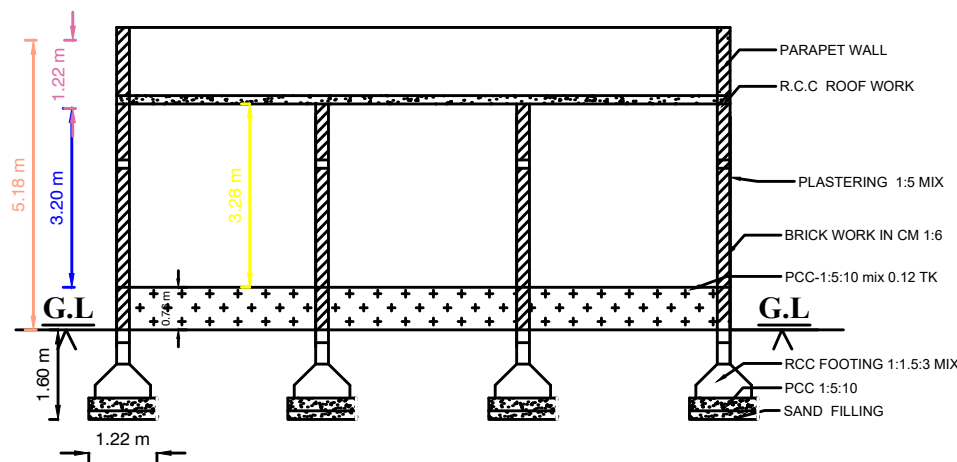
SECTION"AB"
