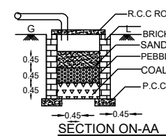
SECTION ON-AA
