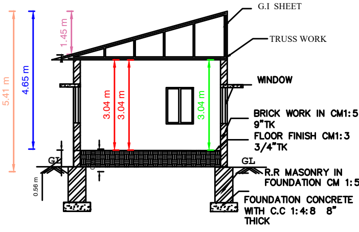
SECTION " AB "
