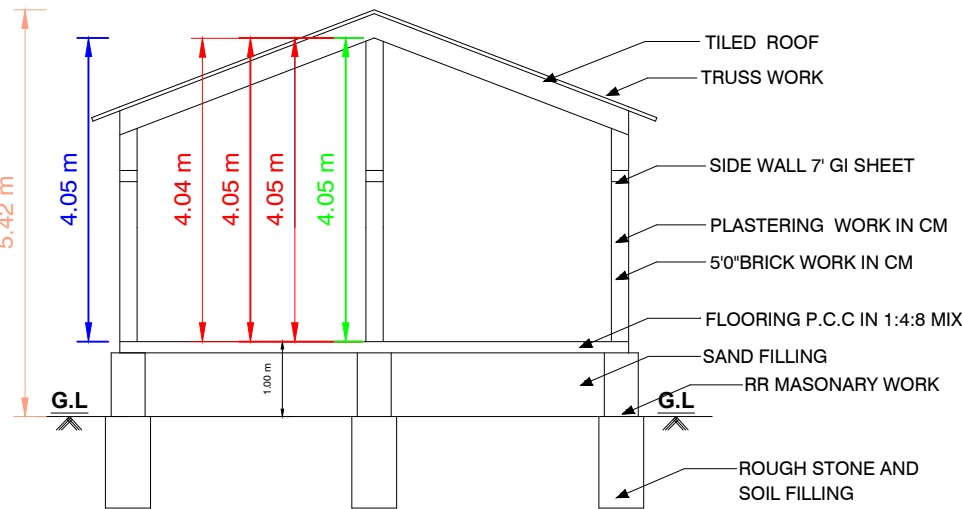
SECTION"AB"
