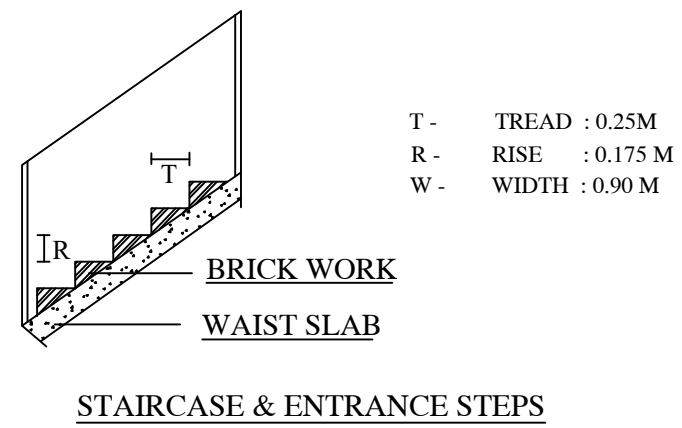
STAIRCASE & ENTRANCE STEPS
