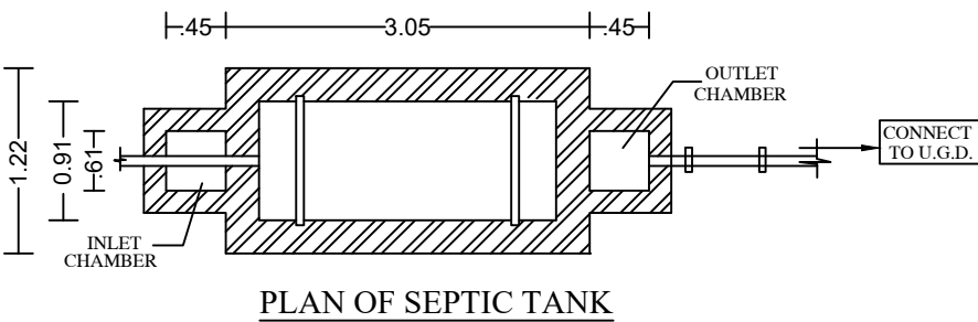
PLAN OF SEPTIC TANK
