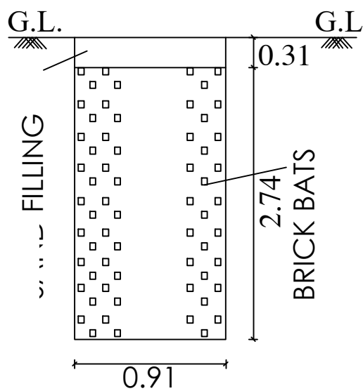
RAINWATER COLLECTION PIT
