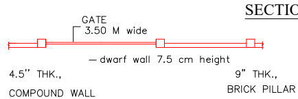
COMPOUND WALL PLAN
