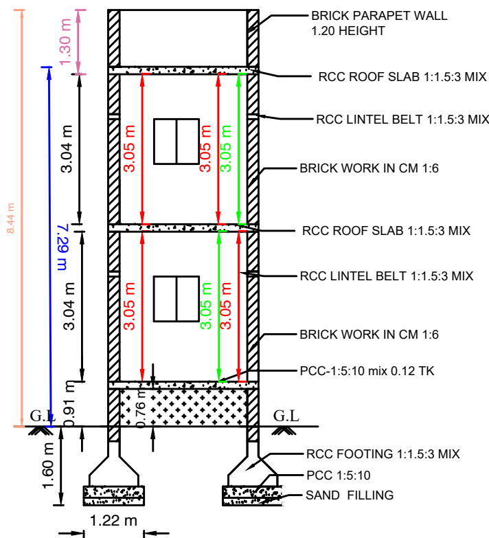
SECTION "AB"
