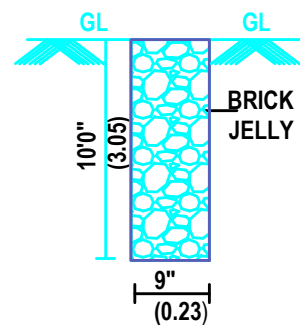
PERCUSSION PIT
