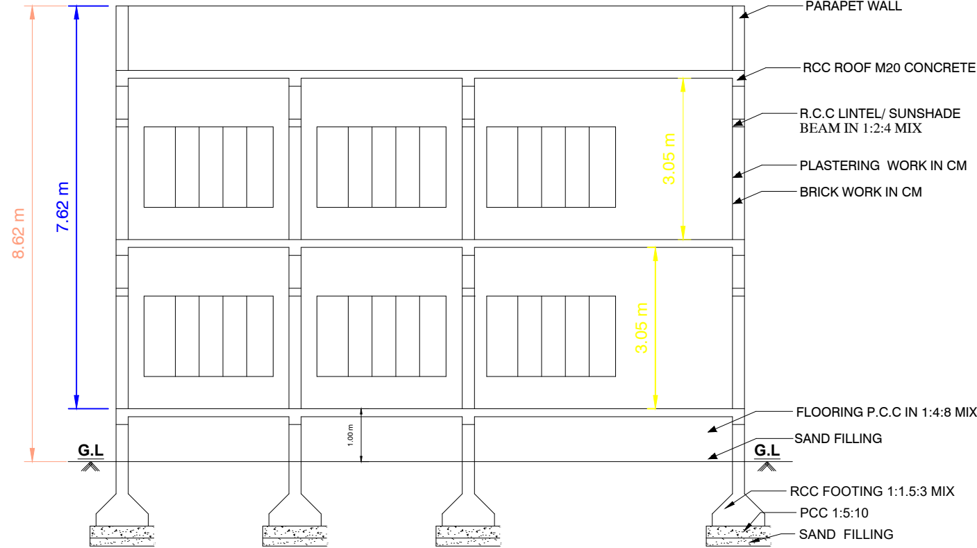
SECTION"AB"
