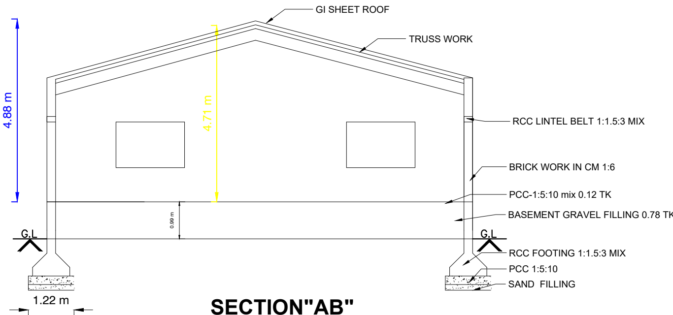
SECTION"AB"
