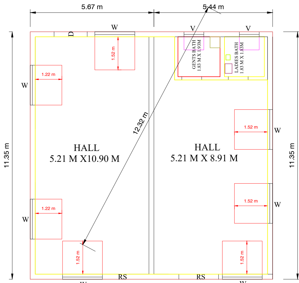
PLAN
