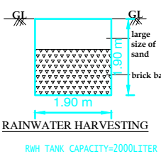
RAINWATER HARVESTING RW TANK CAPACITY=2000LITER
