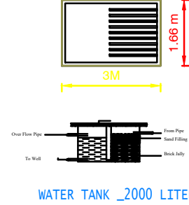
WATER TANK _2000 LITER
