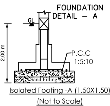
Foundation Detail - A (Not to Scale)
