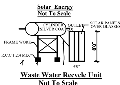
Waste Water Recycle Unit Not To Scale
