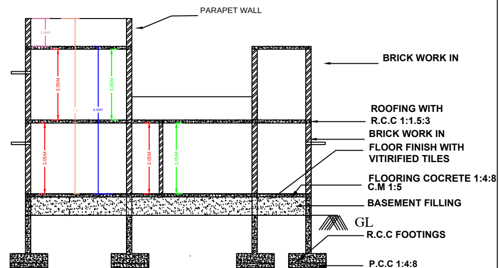
SECTION ON "BB1"
