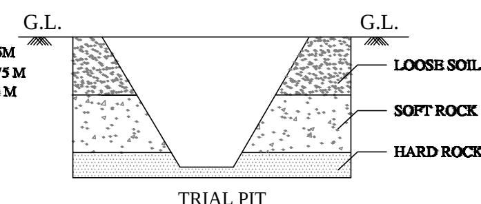
TRIAL PIT
