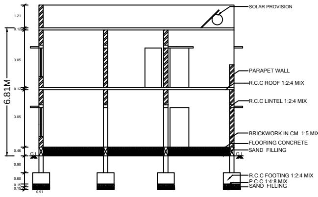
SECTION ON 'ABC'
