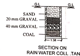
RAIN WATER COLL. TANK
