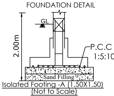
FOUNDATION DETAIL
