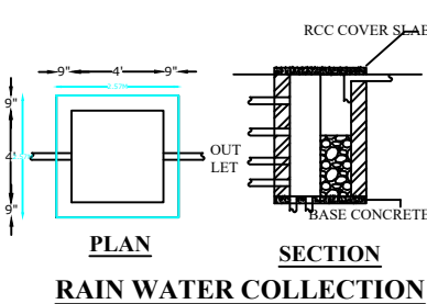
RAIN WATER COLLECTION PIT DETAILS
