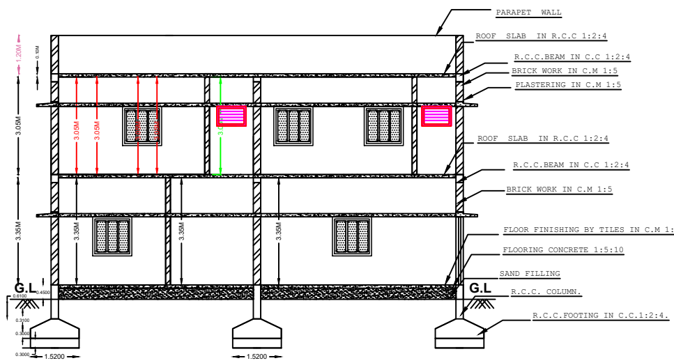
SECTION ON - XY.
