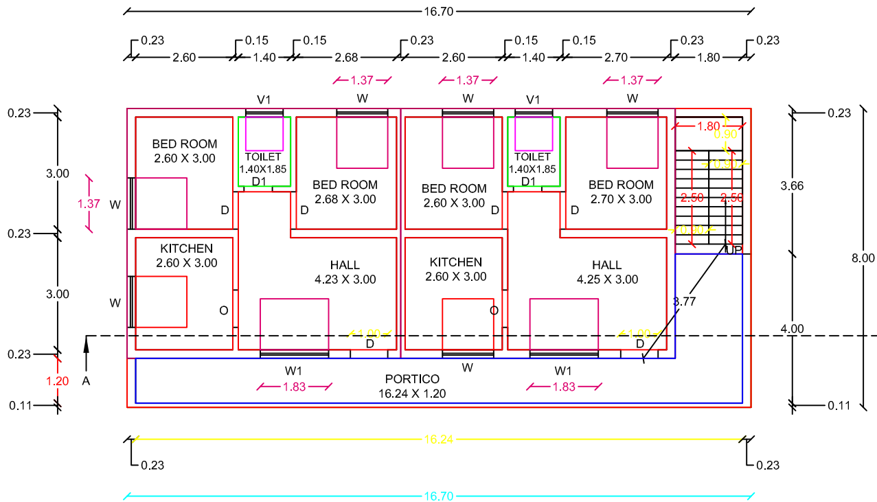
FLOOR-GROUND
