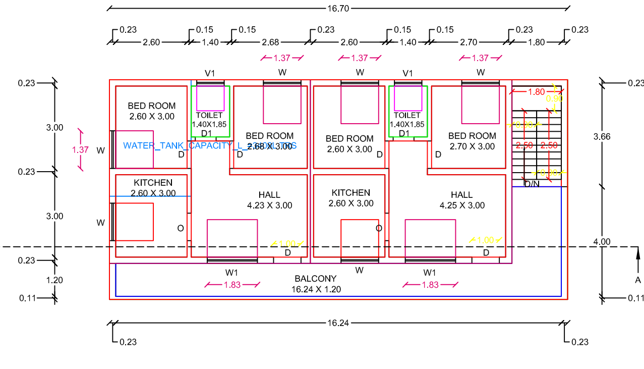
FLOOR01
