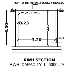
RWH SECTION
