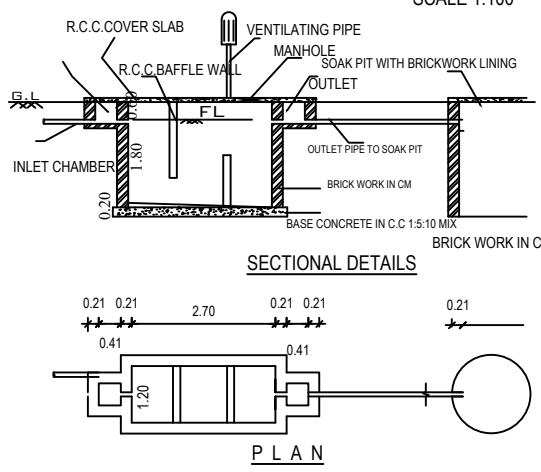
DETAILS OF SEPTIC TANK WITH SOAKPIT
