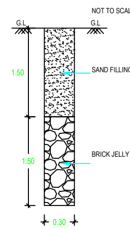
RAIN WATER PERCUSSION PIT
