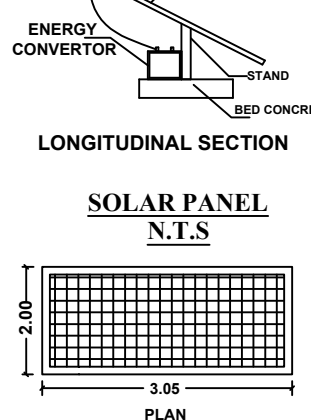
SOLAR BOARD
