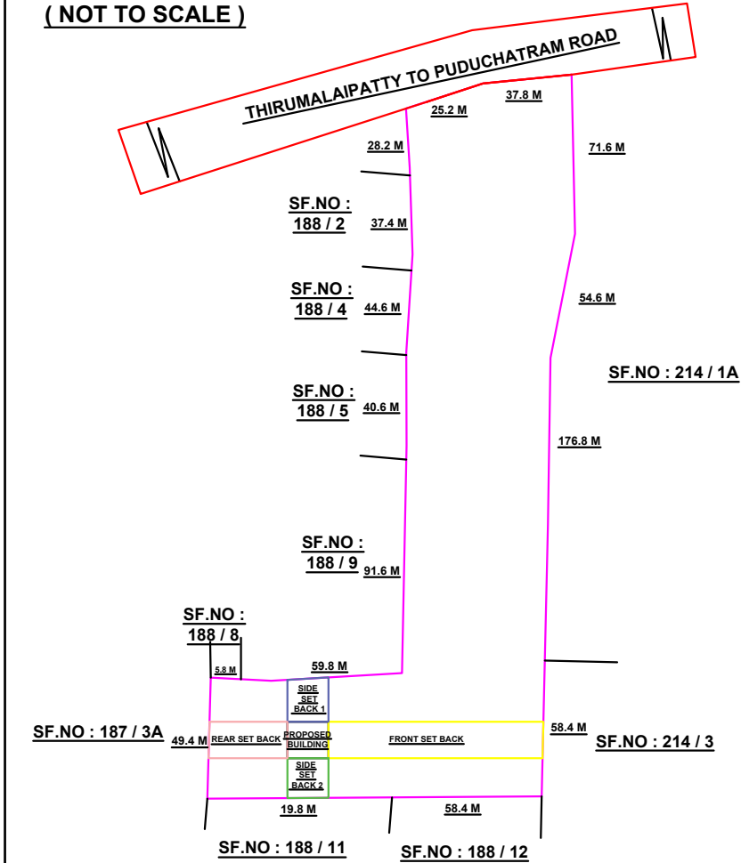
TOPO PLAN
