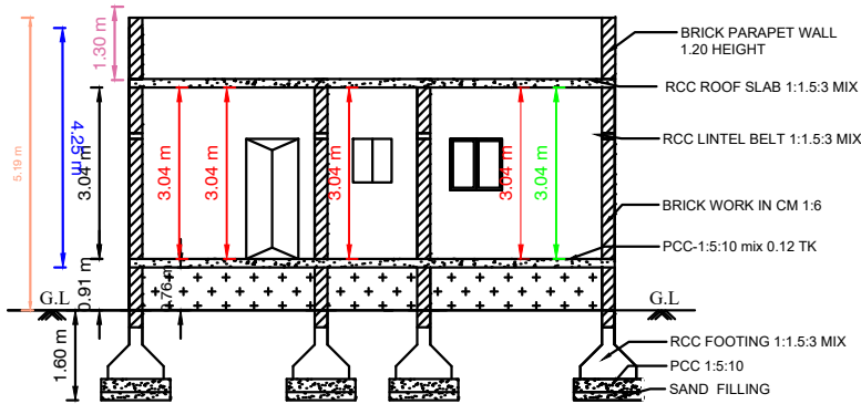
SECTION "AB"
